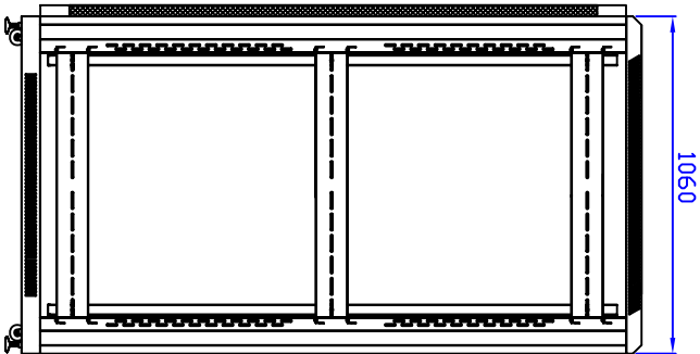
Side View with door removed
