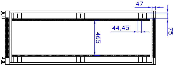
Front View with door removed
